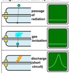
Principle of Geiger-Müller tube operation
